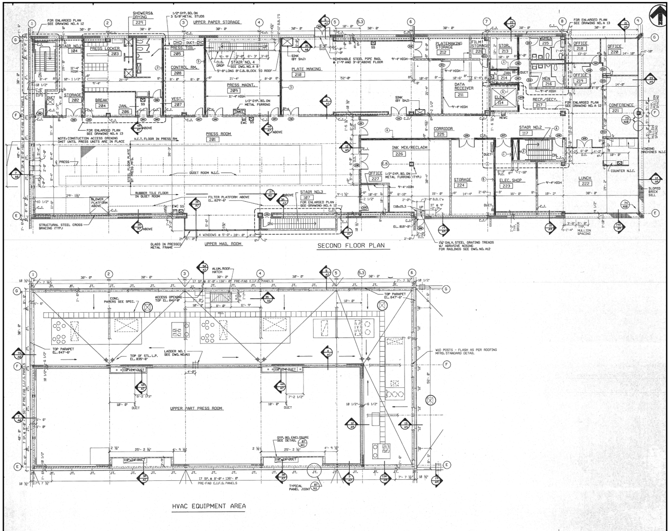
2nd Floor Plan and HVAC
