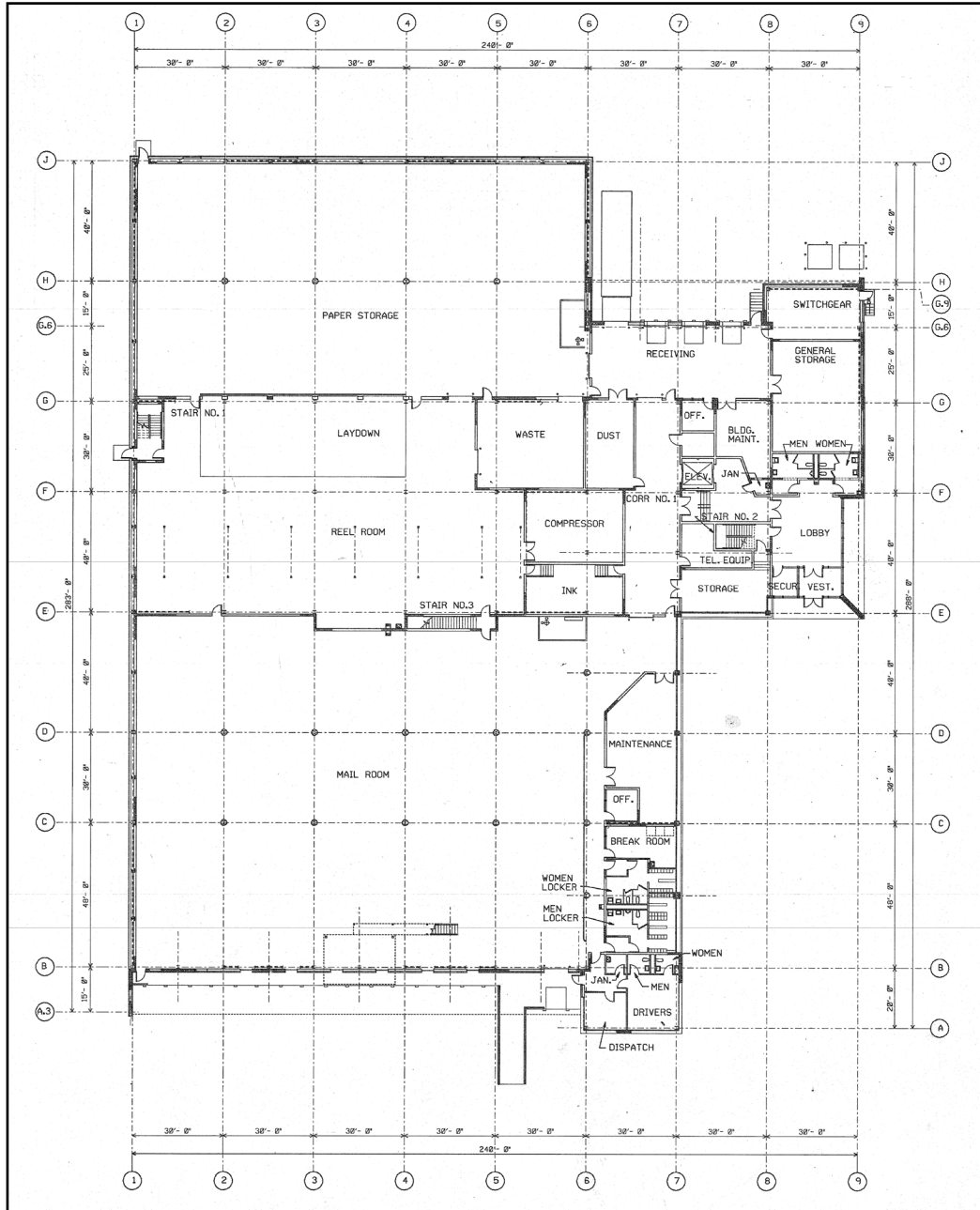
1st Floor Master Plan
